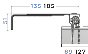
1340 adjustable face fix brackets
