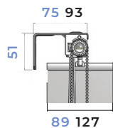
Face fix brackets. 1304: 89mm 1300: 127mm
