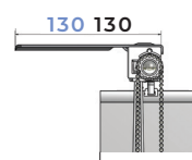
Extension top fix brackets. 1342: 80mm/180mm; 1341: 130mm/230mm; 1351: 160mm/260mm
