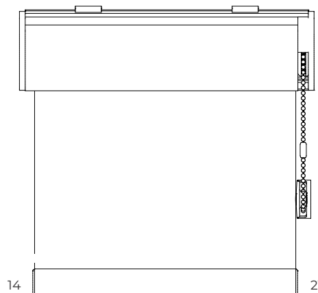
45° standard metal bracket top fix front view
