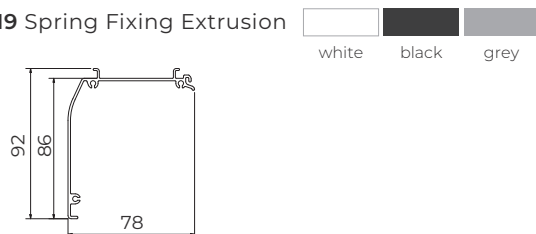
R3522 Profile Fascia
