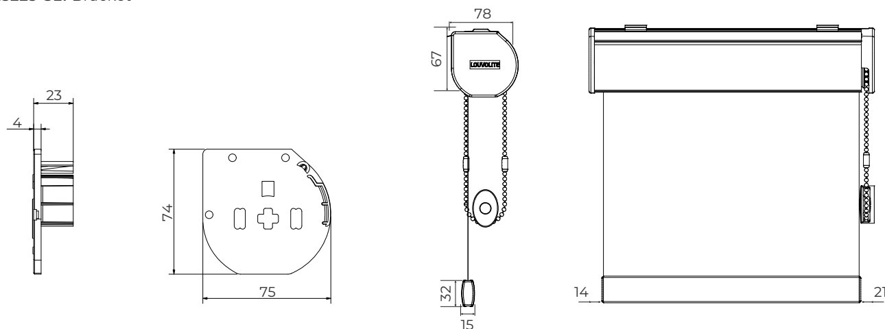
40° standard metal bracket top fix & cover
