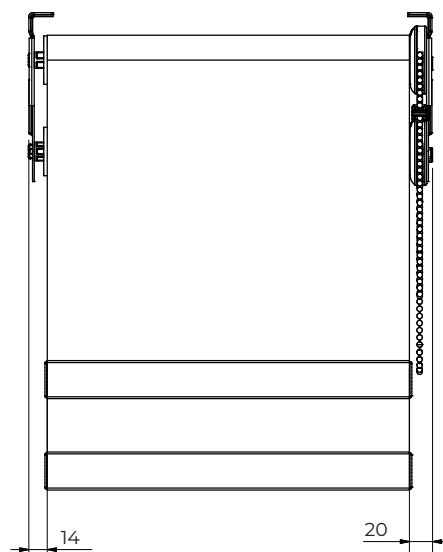
40° double metal bracket top fix front view
