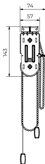
40° double metal bracket top fix
