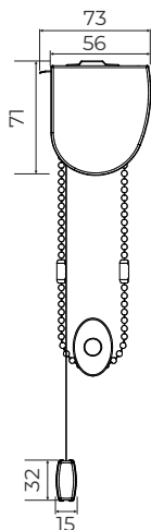
40° standard metal bracket top fix & 70mm cover
