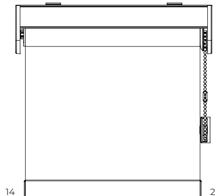
40° standard metal bracket top fix front view
